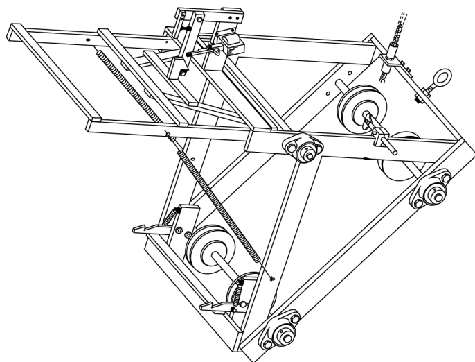
FIG. 2 Platform Assembly
